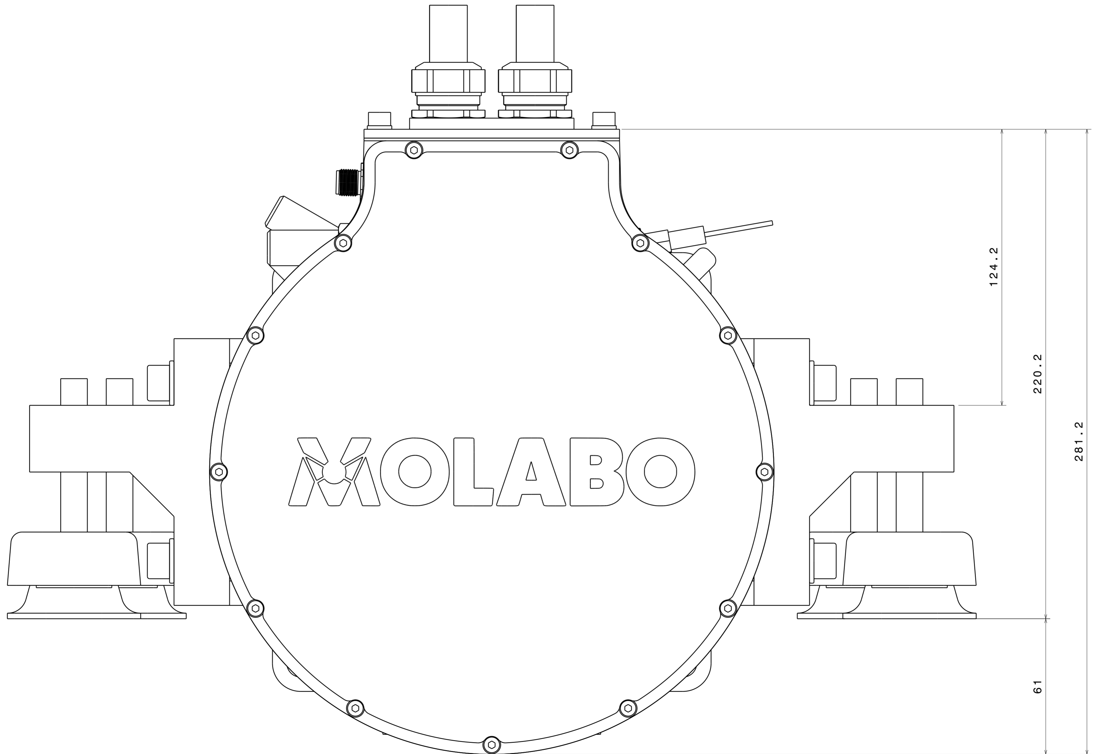
Front View assembled (high)
