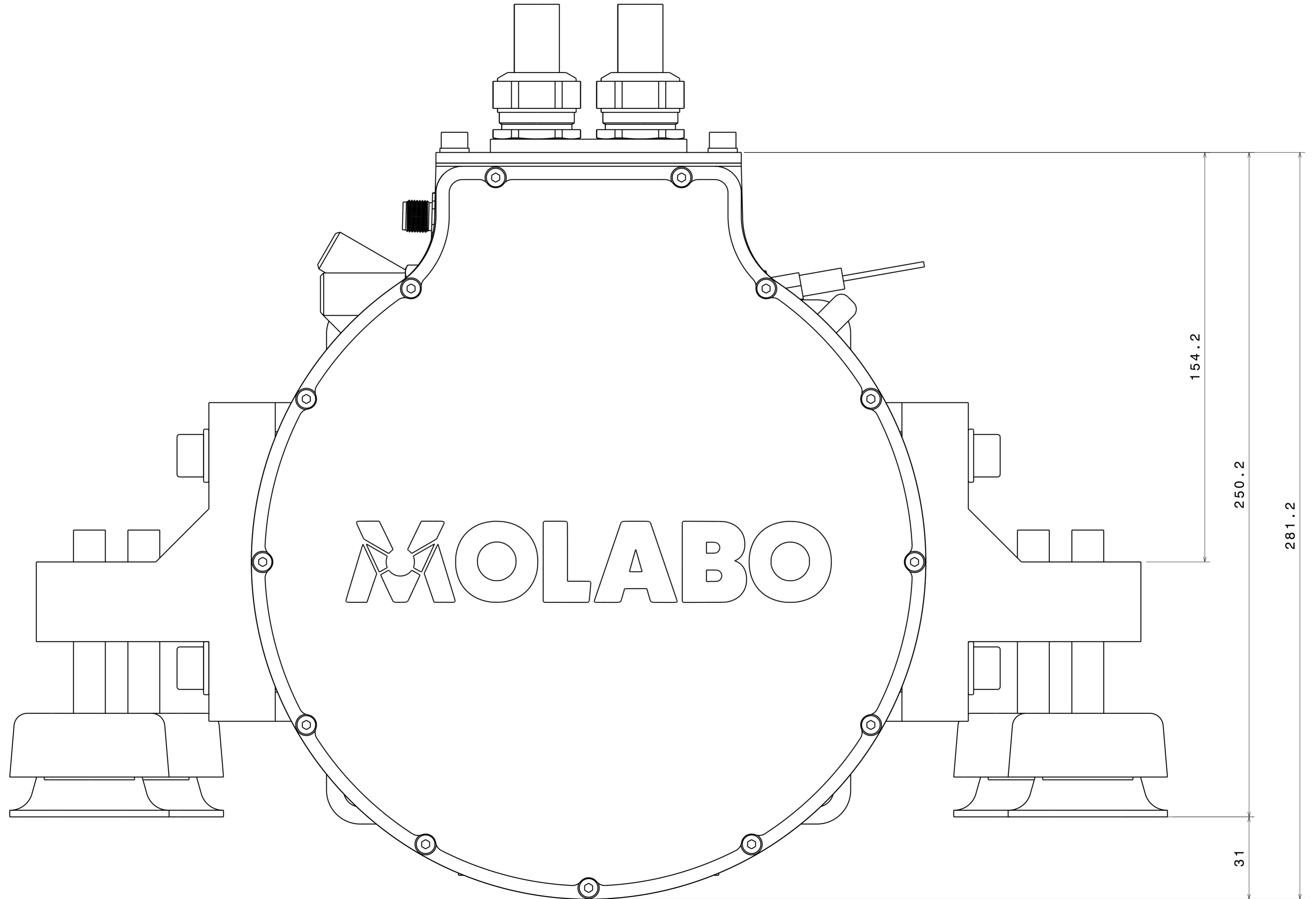
Front View assembled (low)
